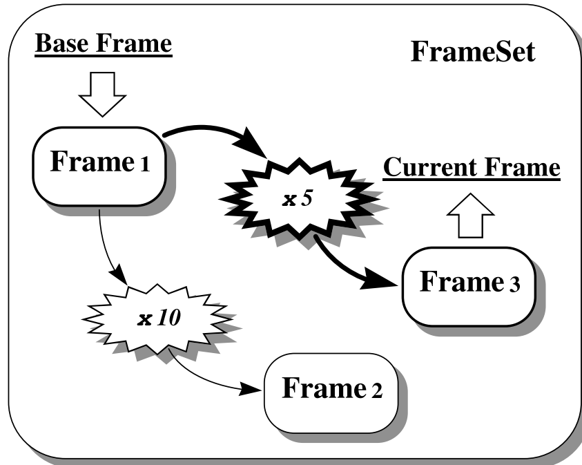
Figure 14: An example FrameSet, in which Frames 2 and 3 are related to Frame 1 by multiplying its coordinates by factors of 10 and 5 respectively. The FrameSet's Base attribute has the value 1 and its Current attribute has the value 3. The transformation performed when the FrameSet is used as a Mapping ( i.e. from its base to its current Frame) is shown in bold.
