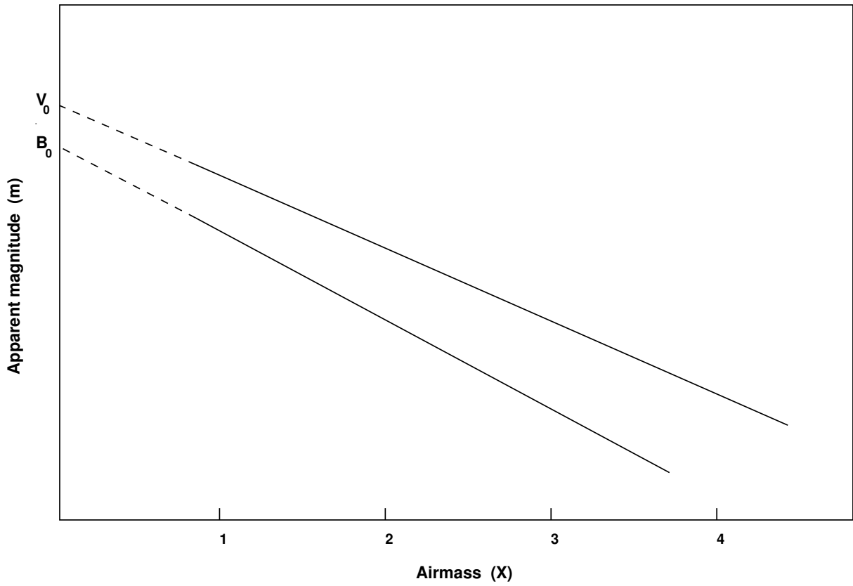
Figure 4: How to determine atmospheric extinction coefficients by plotting apparent magnitudes against air mass throughout the night
