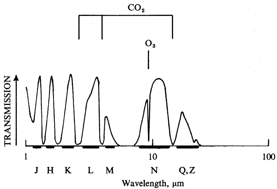
Figure 5: Atmospheric transmission at infrared wavelengths. The windows where the atmosphere is largely transparent are marked. The short-wavelength windows correspond to bands in the JHKLM photometric system. Note the additional N , Q and Z windows at longer wavelengths. Adapted from Allen[2]
