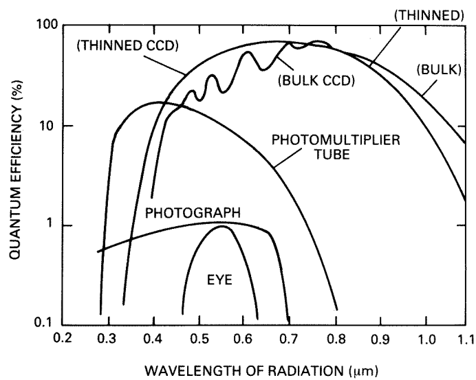
Figure 3: The sensitivity or quantum efficiency as a function of wavelength for various types of detectors. The quantum efficiency is simply the fraction of incident photons which are detected. Here it is plotted on a logarithmic scale. Thinned and bulk CCDs are simply different types of CCDs. Photomultiplier tubes are used in photoelectric photometers. Note that CCDs are more sensitive to red light than photomultiplier tubes. Adapted from McLean[56]
